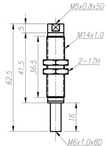
ELF-15-M14
