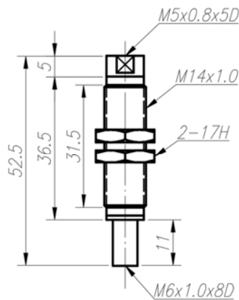
ELF-10-M14
